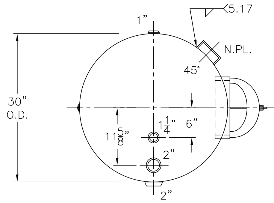
VIEW W/OUT SUPPORTS
